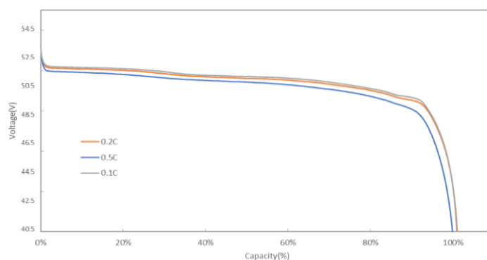
Voltage vs. Discharge Capacity Percentage with Different Current Rate
